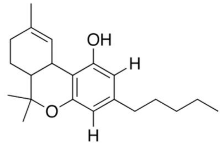
Tetrahydrocannabinol (THC)
