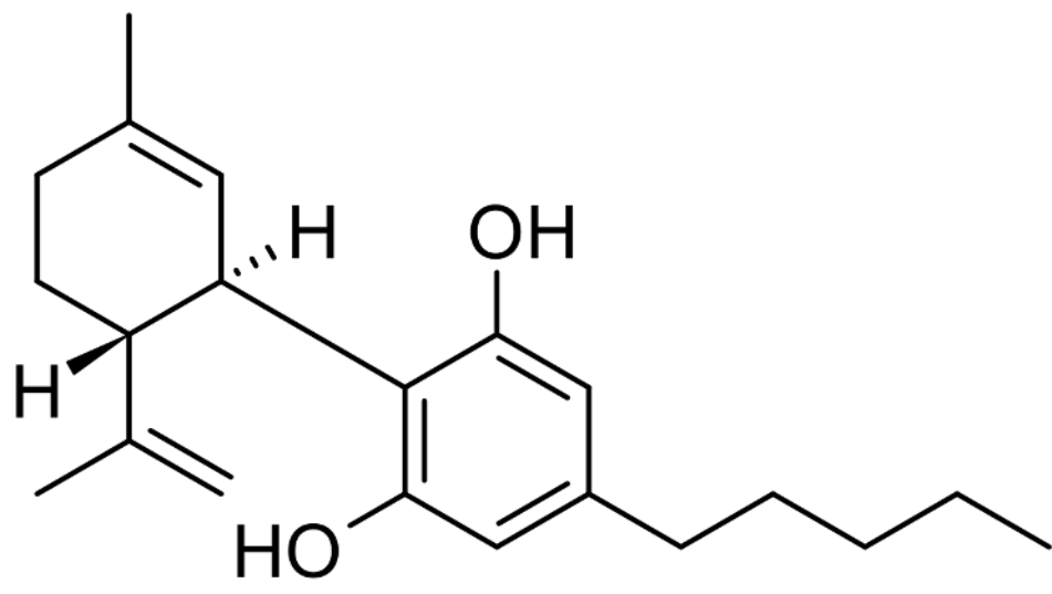
Cannabidiol (CBD)
